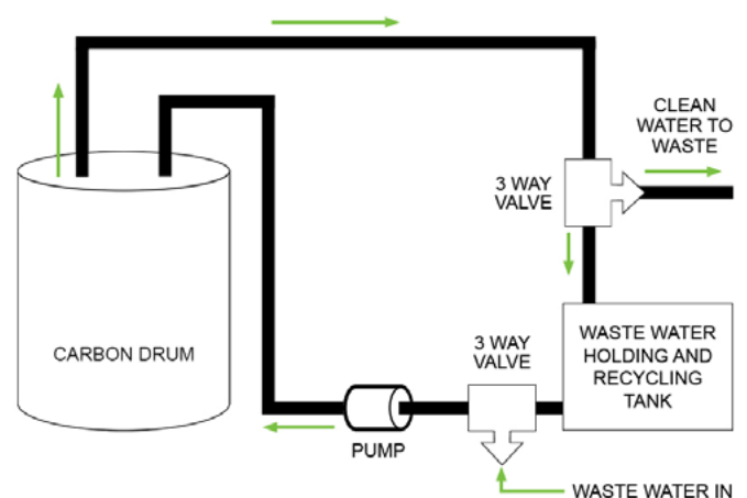
Carbon filtration general flow diagram
